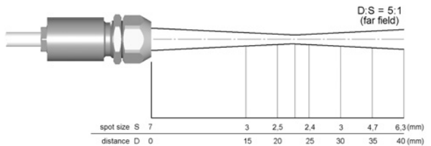
2:1 optics with CF-lens
